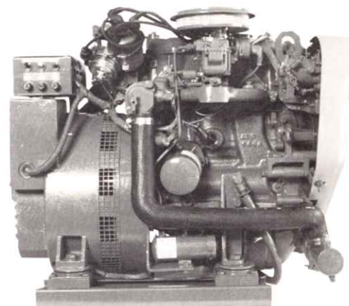
The 9 KW features very compact dimensions and simplicity of design.
